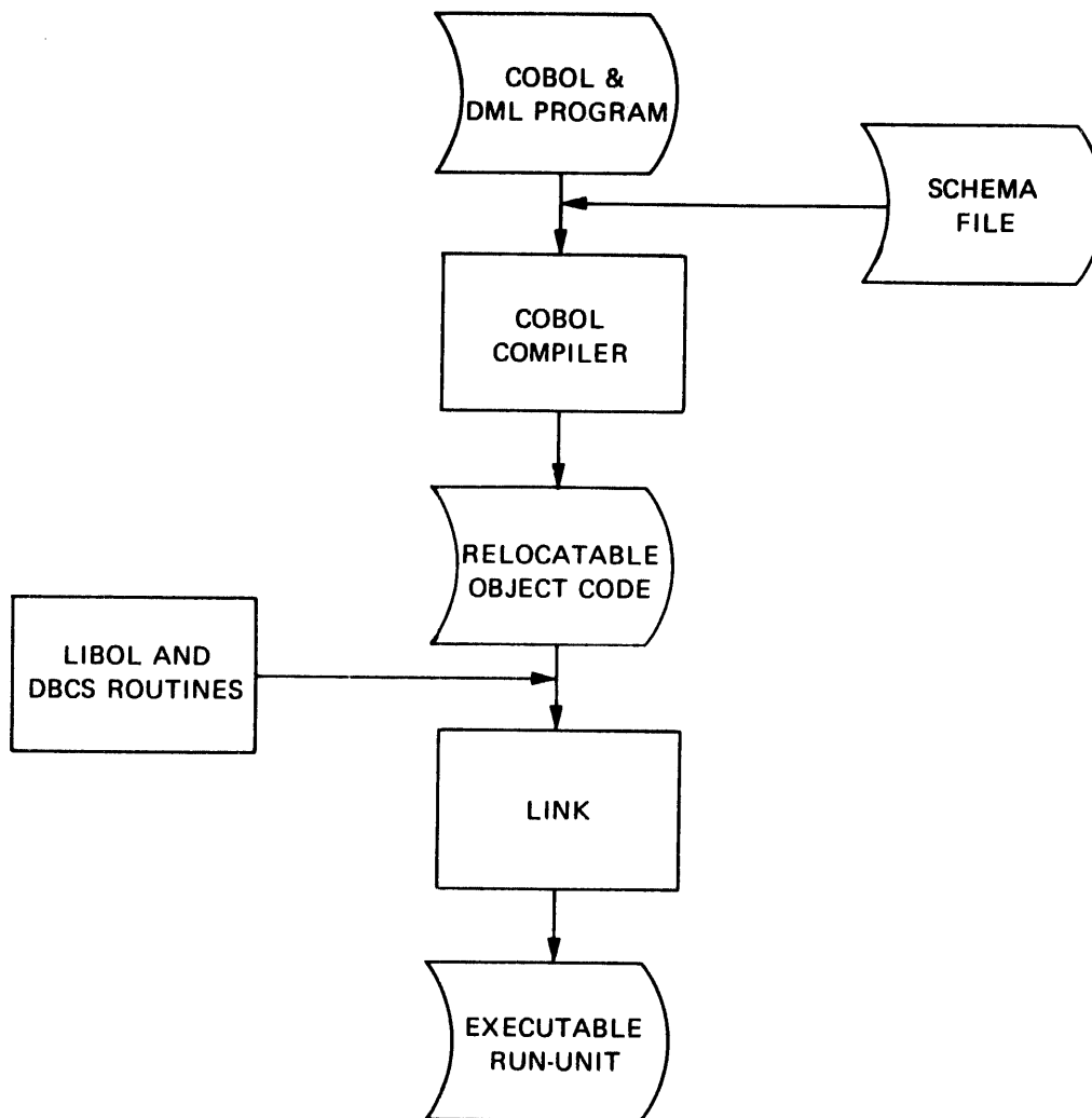
Figure 4-1 Program-Building Process for COBOL with DML
