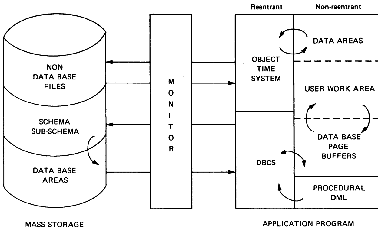
Figure 1-4 Data-Base Environment
